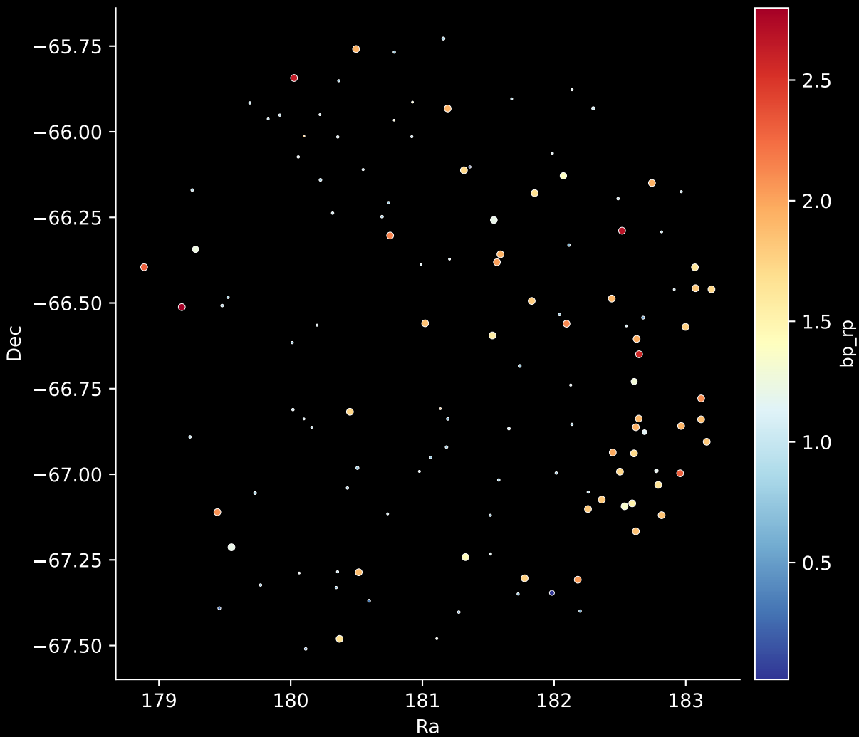
APOGEE DR17 Field: [277-33-O_TESS] Stars: 126
