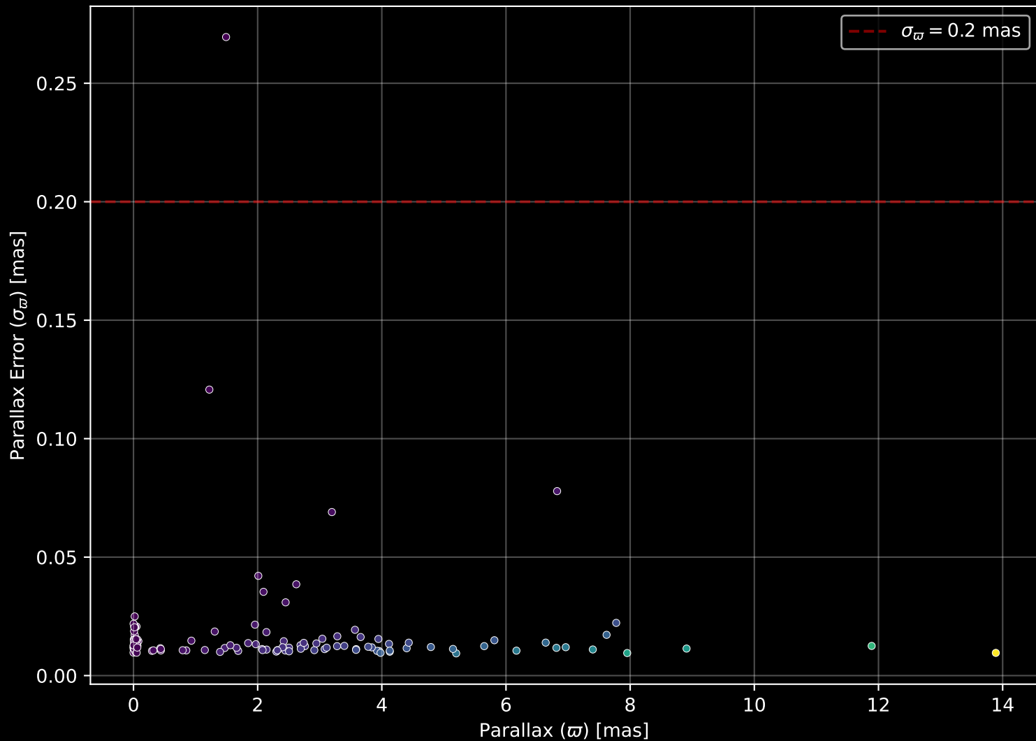
APOGEE DR17 Field: [277-33-O_TESS] Parallax Quality (n= 126)
