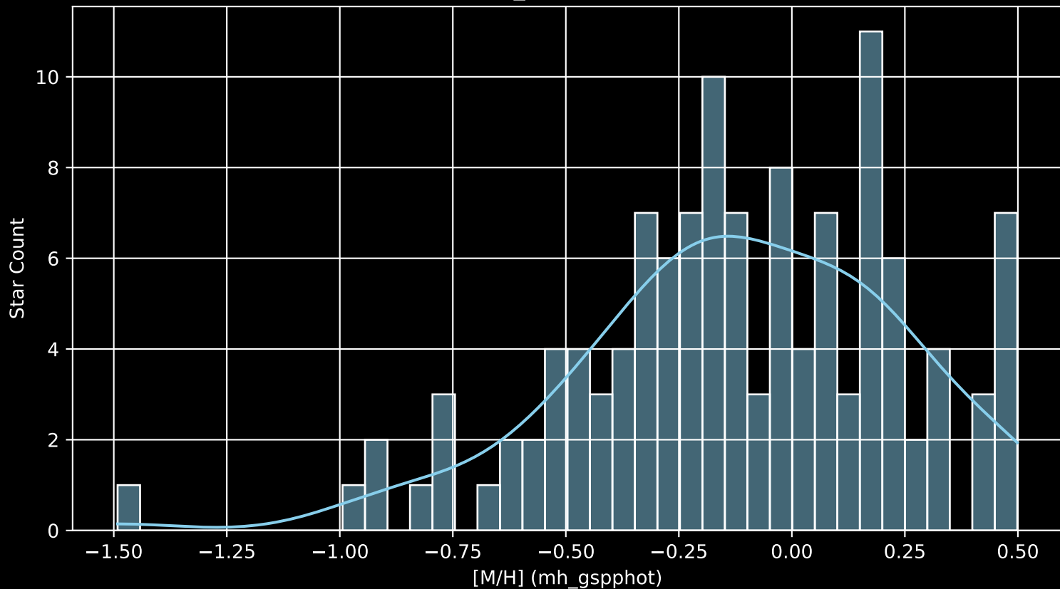
APOGEE DR17 Field: [277-33-O_TESS [M/H] (mh_gspphot) (n= 123)
