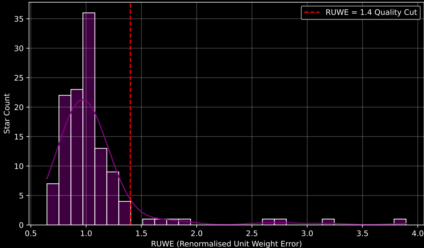
GAPOGEE DR17 Field [277-33-O_TESS] RUWE Distribution (n= 122)
