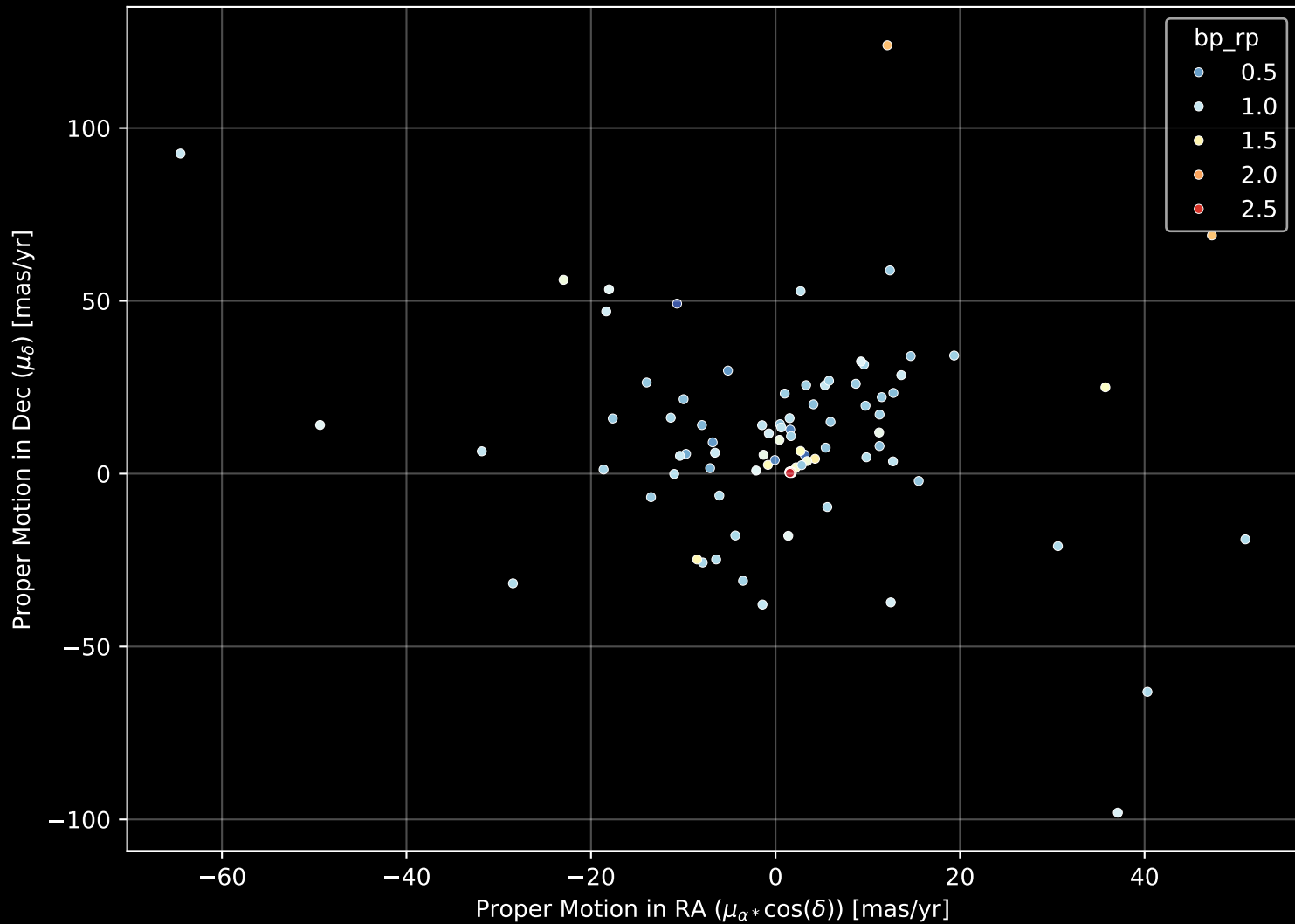
APOGEE DR17 Field: [277-33-O_TESS] Proper Motion Diagram (n= 126)
