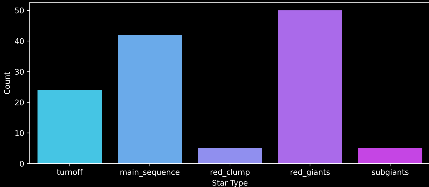
APOGEE DR17 Field: [277-33-O_TESS] Count plot of Star Type
